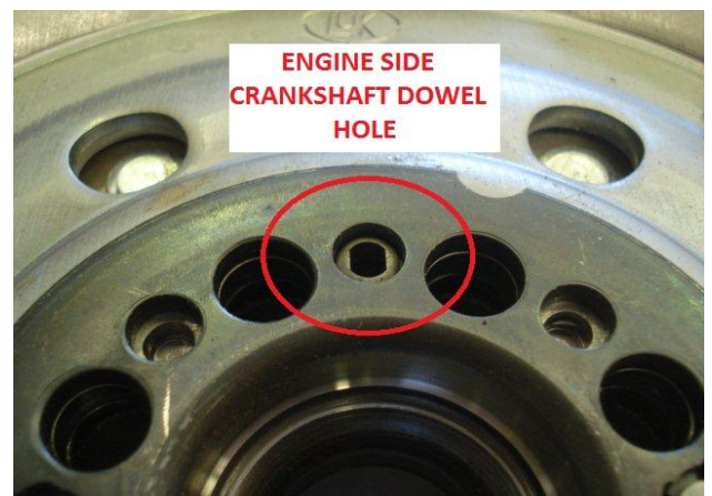
Figure 2 (Engine Side)
